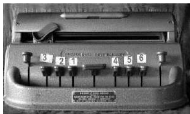
Illustration 21: Machine Perkins
